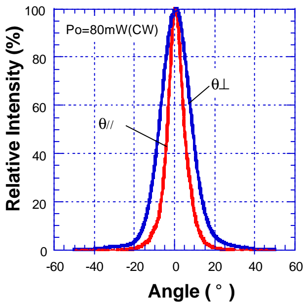
Far-Field-Patterns
